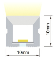
Unit: mm Cross section
