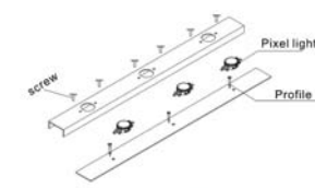
B. Profile installation
